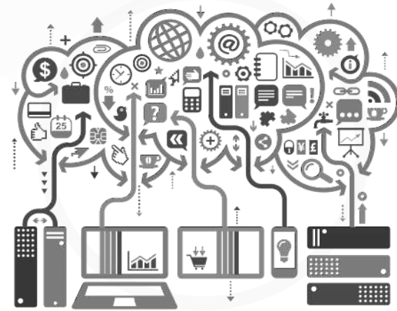
Big Data
